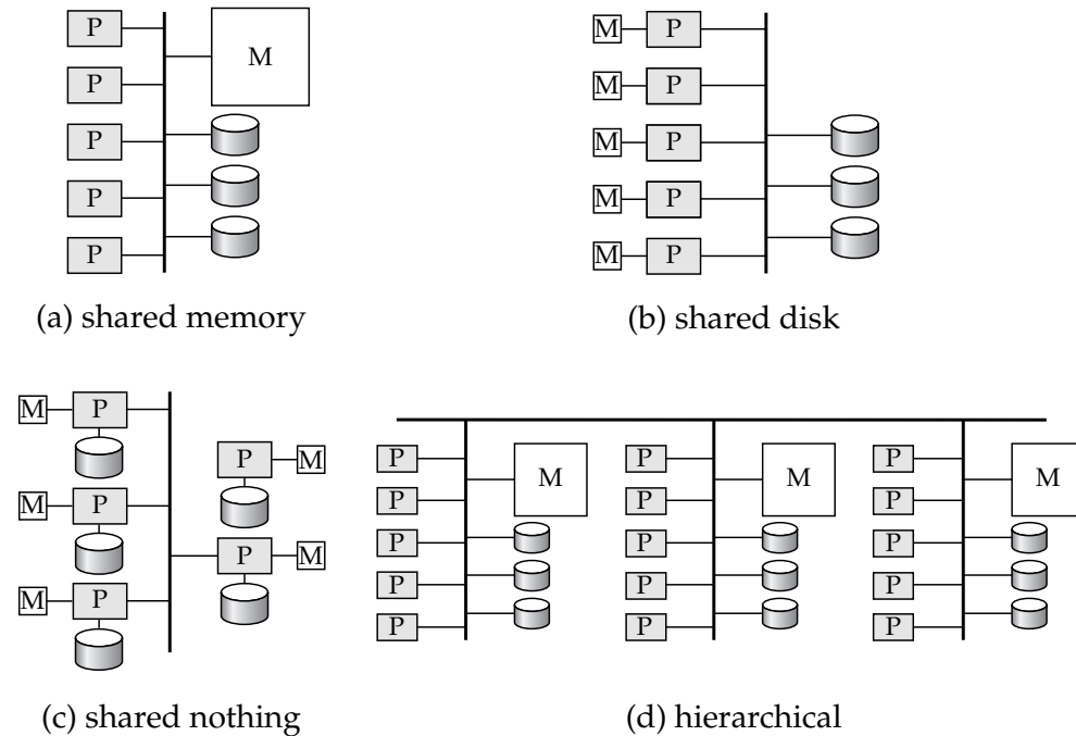
Figure 18.8 Parallel database architectures.
