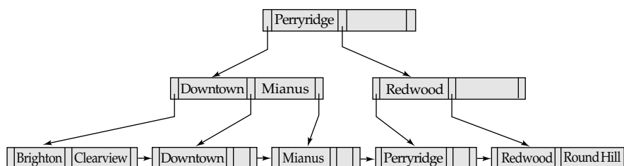
Figure 16.22 Insertion of “Clearview” into the B + -tree of Figure 16.21.
